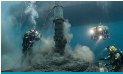
Underwater Concrete
